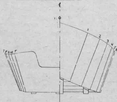
FRAME STATION 1 LOOKING AFT NOTE: THIS FRAME MUST BE MOVED TO AFT SIDE
