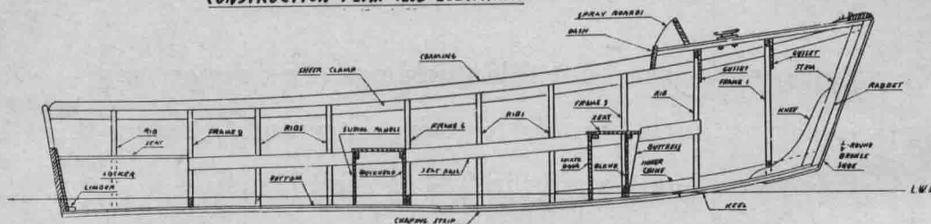
CONSTRUCTION PLAN AND ELEVATION
