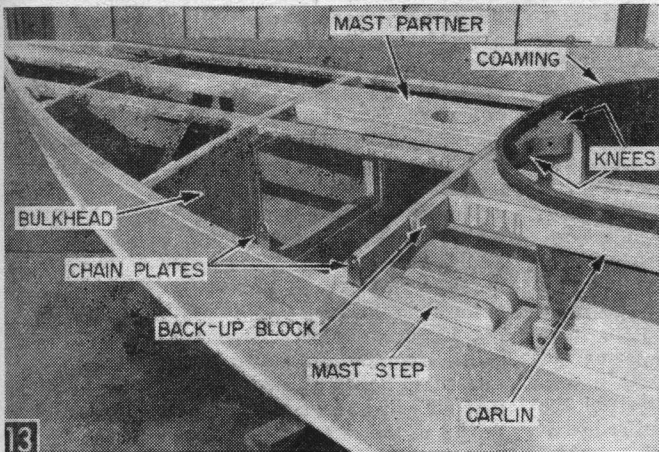
13 Forward view of hull showing location of parts under the decking.
