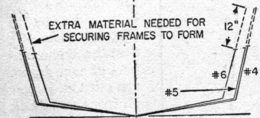
LAYOUT FRAMES 4, 5 & 6 ON BACK SIDE OF PAPER
