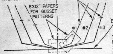
FULL SIZE FRAME LAYOUTS (SEE FIG. 4 FOR DIMENSIONS)
