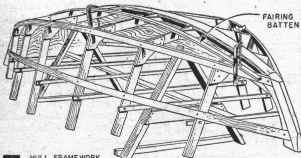
6 HULL FRAMEWORK AND BUILDING FORM
