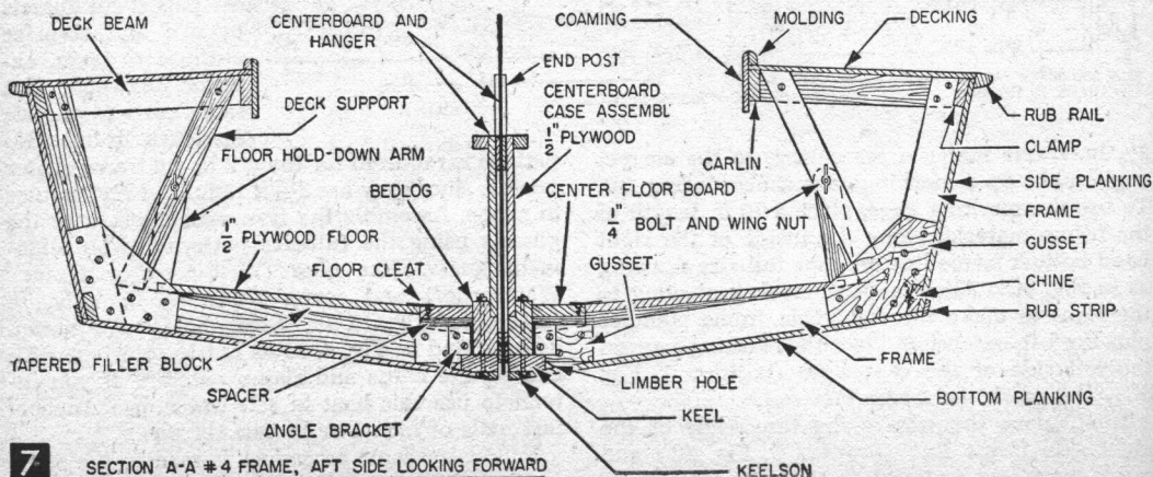
SECTION A-A #4 FRAME, AFT SIDE LOOKING FORWARD
