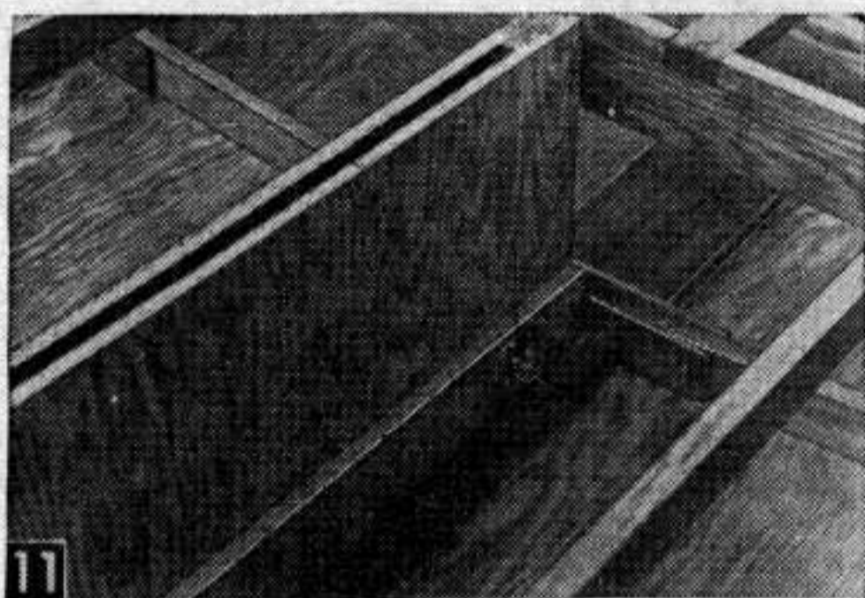
Centerboard well screwed in and caulked at bed logs. Make sure sides and bed logs are square with keel.
