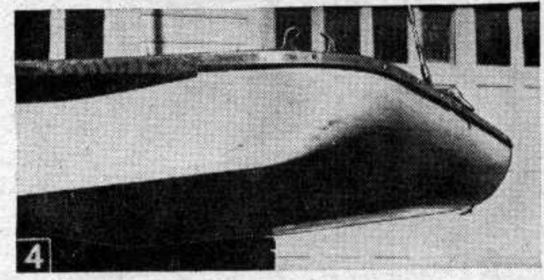
Fig. 2. Aft end and side deck framing just before planking. Note spacing of two center battens about centerline. Fig. 3. Prow framing before decking. Mast step, prow nose are in and ready for plywood decking. Fig. 4. Smooth lines of prow nose.
