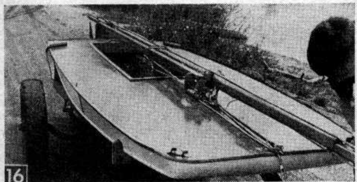
With mast lashed to top of deck fittings, Tern makes a neat package for convenient trailering to your favorite inland lake.
