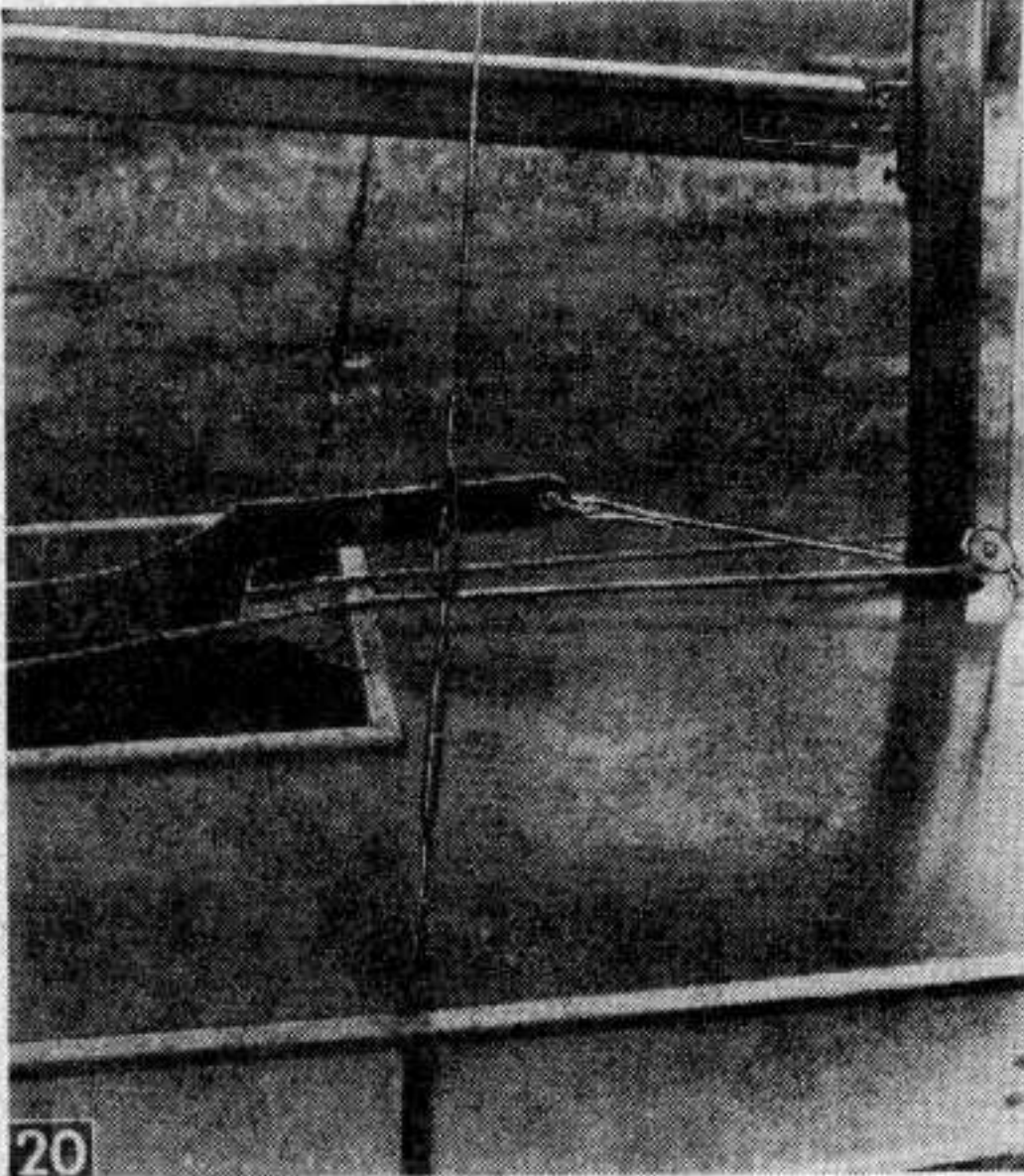
20 Rigging for centerboard with the board in Up position. Noteworthy are mast side stays and boom fittings.
