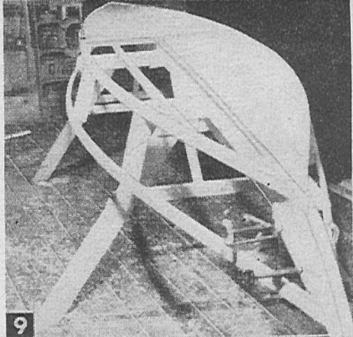
One 4 x 8 ft. plywood panel cut into three pieces as in Fig. 8 covers entire bottom. Half of aft end remains to be covered here.
