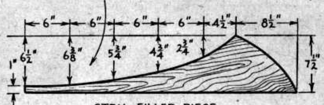
STEM FILLER PIECE 1/4" PLYWOOD - 4 REQUIRED
