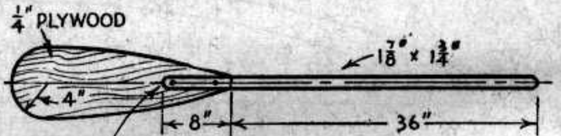
SLOTTED CANOE PADDLE
