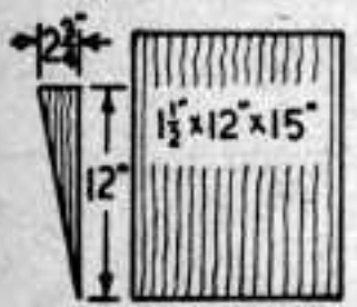
MOTOR BOARD
