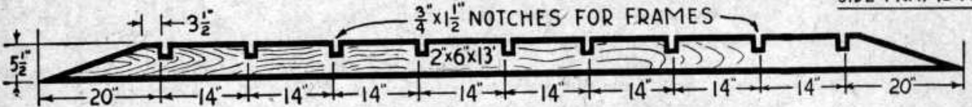
FORM FOR ASSEMBLING FRAMES
