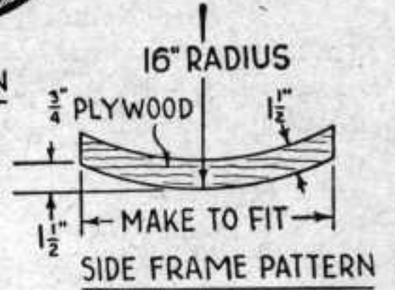
CANOE BOW CONSTRUCTION
