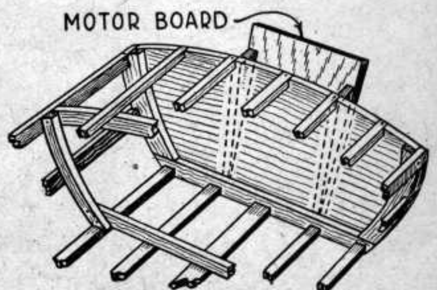
TRANSOM OF OUTBOARD MODEL
