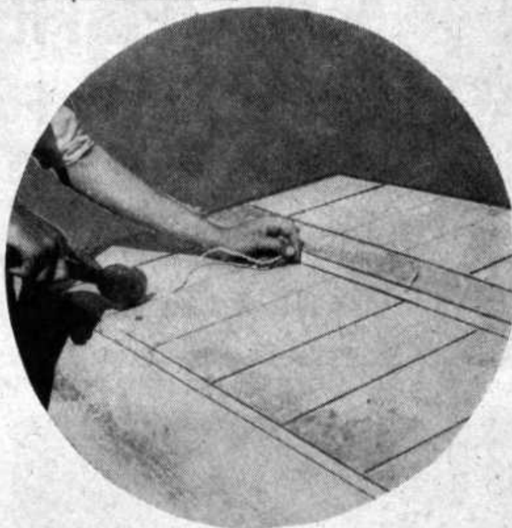
Caulking the crosswise planked seams.
